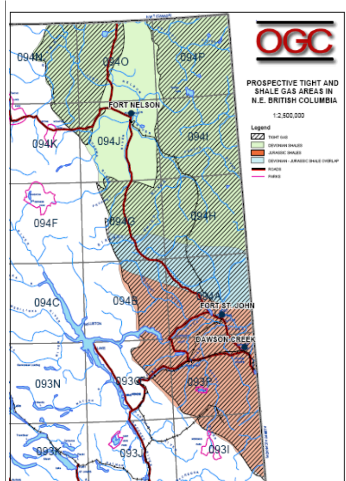
Figure 2: Tight and shale gas areas in B.C.
