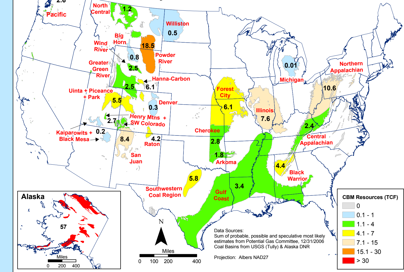
US Coalbed Methane Resources (TCF) By Basin, December 2006
